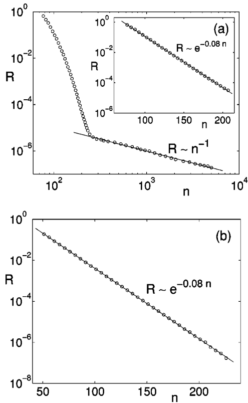
FIG. 2. Time decay for map (1) with \lambda=4.0 , in the interval [x_0, x_0 + 10^{-7}] . (a) \nu=0 , x_0=0.577\ 005\ 0 . The inlet corresponds to the initially exponential decay. (b) \nu=0.001 , x_0=0.576\ 000\ 6 .
