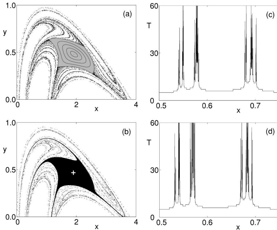
FIG. 1. Phase-space structure and time-delay function for map (1) with \lambda = 4.0 . (a) \nu = 0 : KAM island (in gray), scattered orbits (in black), and the fractal boundaries of the scattered orbits (in black). (b) \nu = 0.01 : captured orbits (in black) and scattered orbits (in black). The plus sign is the fixed point attractor. (c), (d) Time delay in the conservative and dissipative cases of (a) and (b), respectively. T is the time taken by particles to reach \sqrt{x^2 + y^2} \geq 100 .
